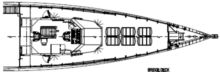
BRIDGE DECK
