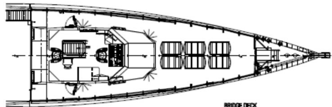
BRIDGE DECK
